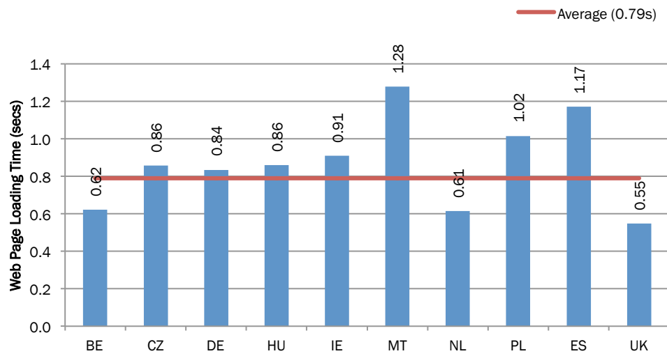
Figure EU.2-26: Web Page Loading Times of cable technology during peak periods, split by country
