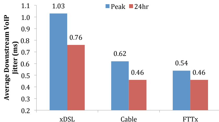
Figure EU.1-32: Peak period and 24-hour Downstream VoIP Jitter, split by technology (lower is better)
