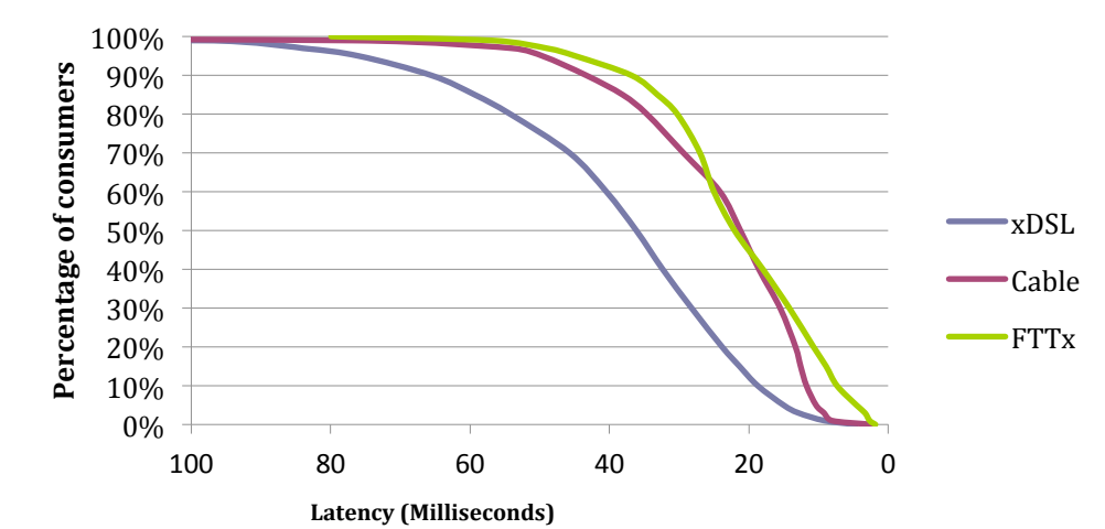
Figure EU.1-14: Cumulative Distribution of Average Latency, split by technology (lower is better)
